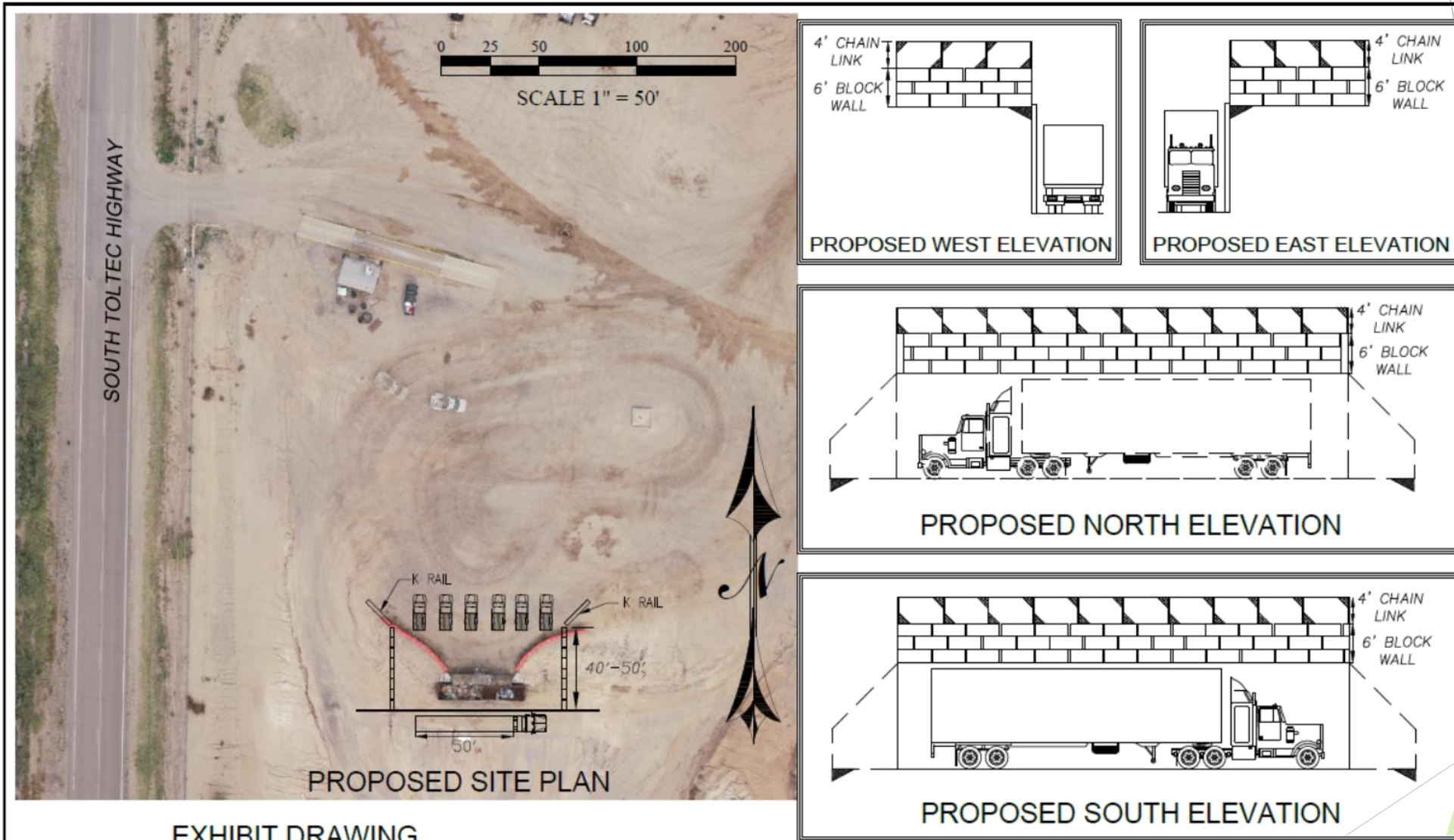
EXHIBIT DRAWING
